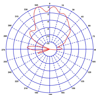
2000 MHz Elevation
