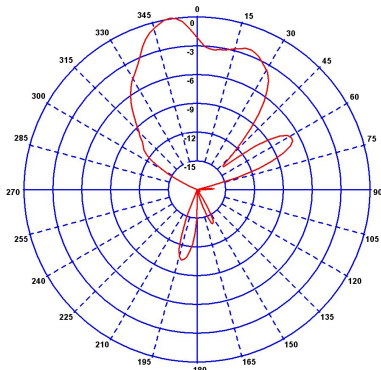
2000 MHz Elevation
